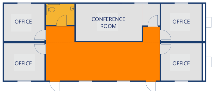
24' X 60' 4 OFFICE, CONFERENCE ROOM AND RESTROOM
